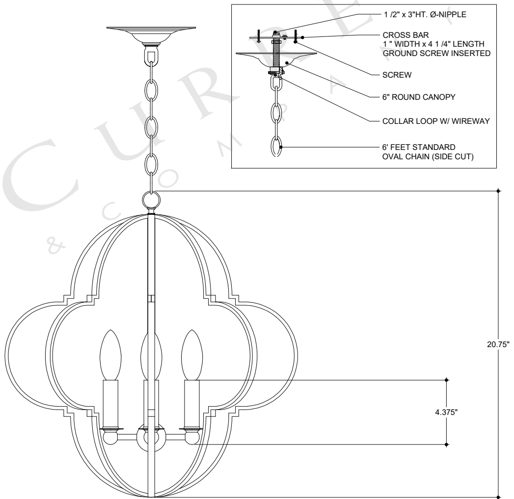
FRONT VIEW
